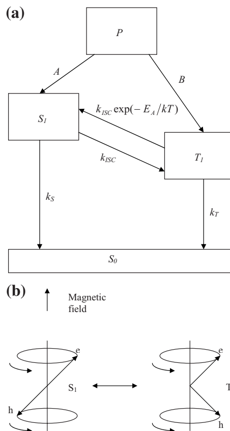
FIG. 5. (a) A schematic diagram of the excitation and recombination pathways in an organic molecule. The excitation pump P produces no triplets under illumination (i.e., B=0 ), but in electrical pumping, A=0.25 and B=0.75 . (b) A vector diagram illustrating the increased singlet m=0 triplet intersystem crossing due to a magnetic field.
