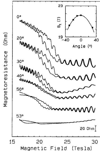
Fig. 6. Angular dependence of the high field (MR) showing a drop (“kink”) in resistance around 22 T; the traces are offset for clarity and the temperature is 490 mK. The inset shows the angular dependence of the “kink” (points) fitted to a \cos^{1/2} \theta dependence (line).
