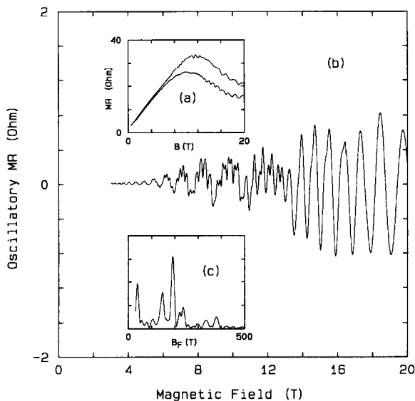
Fig. 1. (a) β''ET 2 AuBr 2 magnetoresistance (MR) at 490 mK for B parallel to b * (upper trace, 0°) and for B tilted 30° from b * about a ' towards c (lower trace). (b) The oscillatory part of the 30° MR. (c) Fourier spectrum of the 0° trace shown in fig. 1(a).
