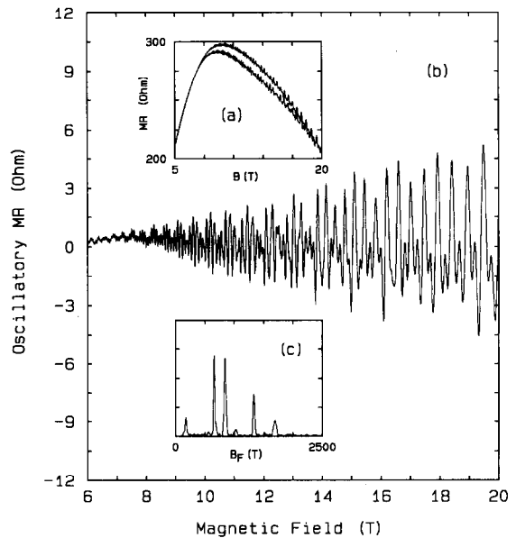
Fig. 4. (a) MR of a sample of \text{ET}_2\text{KHg}(\text{SCN})_4 showing hysteresis; the upper trace is the upsweep, the lower the downsweep. (b) Oscillatory component of MR showing beats and spin-splitting. (c) Fourier spectrum of fig. 4(b) showing two frequencies F1 and F2 plus their harmonics and frequency mixing.
