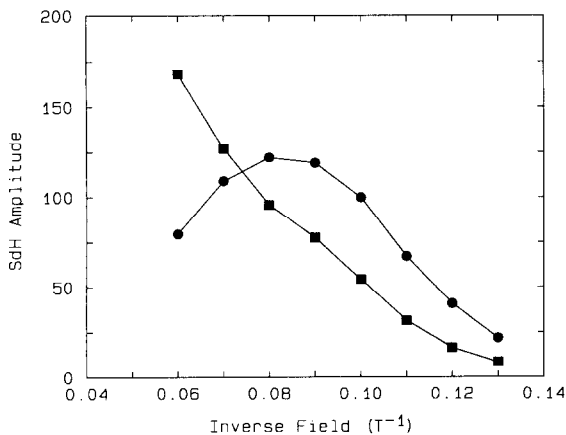
Fig. 5. Fourier amplitudes of F1 and F2 . These points are obtained by transforming within a shifting 0.1 \text{ T}^{-1} wide data window.
