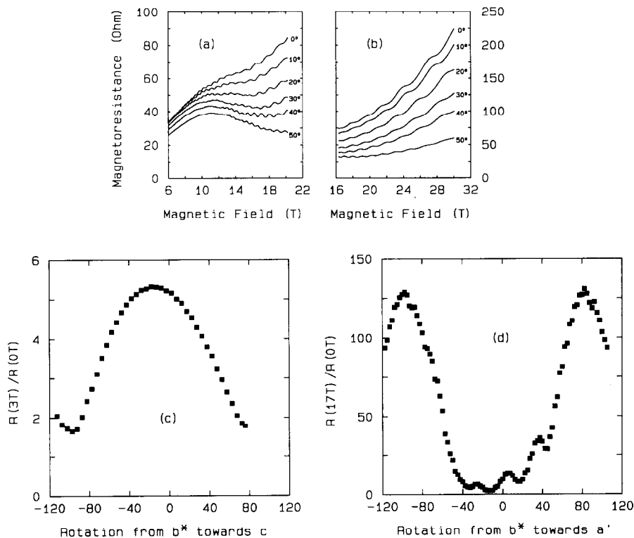
Fig. 2. (a,b) MR as a function of tilt angle about a' ( T = 490 mK). (c) MR at 3 T for tilting about a' axis ( T = 1.7 K). (d) MR at 17 T for tilting about c axis ( T = 1.7 K). In all three cases, the angle \theta denotes the angle between B and b^* .
