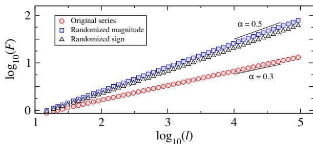
FIG. 5: (Color online) F(\ell) vs. \ell for anticorrelated series ( \alpha_{\text{in}} = 0.3 ) and for surrogate series obtained by means of sign or magnitude randomization: Generate a sign with \alpha_{\text{in}} = 0.3 , decompose it into its magnitude and sign series, randomize the sign or magnitude series and obtain two surrogate series, one multiplying the randomized sign by the original magnitude ( \triangle ) and the other multiplying the randomized magnitude by the original sign ( \square ). Both curves have been obtained for signals with N = 2^{20} and averaging over 200 experiments.
