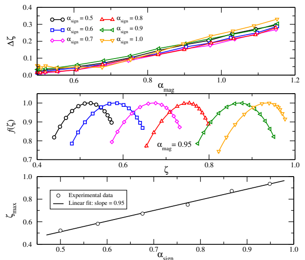
FIG. 11: (Color online) (a) Relation between \Delta\zeta and \alpha_{\text{mag}} of composed series by means of independent magnitudes and signs. \Delta\zeta increases linearly with \alpha_{\text{mag}} when the magnitude series leave the uncorrelated regime ( \alpha_{\text{mag}} > 0.5 ), whereas \alpha_{\text{sign}} does not play an important role in the value of \Delta\zeta . Series are 2^{18} long and results are averaged over an ensemble of 50 series. (b) Example of multifractal spectra of 2^{18} long series with \alpha_{\text{mag}} = 0.95 and \alpha_{\text{sign}} in the interval [0.5, 1] . To obtain the multifractal spectra, the MFDFA analysis (5) has been carried out for moments q \in [-5, 5] . Despite varying \alpha_{\text{sign}} , \Delta\zeta is practically the same for all cases. Spectra are centered in \zeta_{\text{max}} \simeq \alpha_{\text{sign}} . (c) Relation between \alpha_{\text{sign}} and \zeta_{\text{max}} for the multifractal spectra obtained in b). The data were linearly fitted with slope 0.95.
