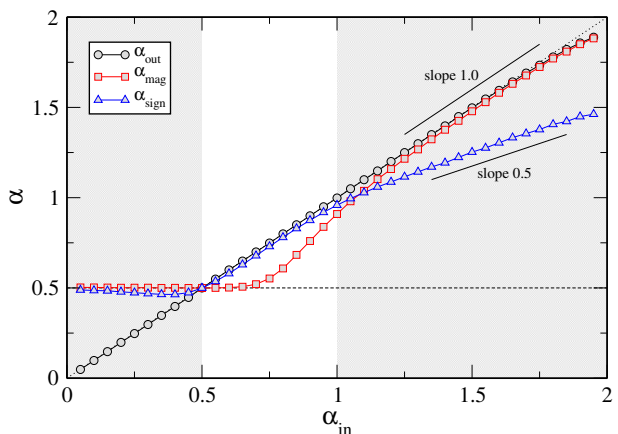
FIG. 3: (Color online) Averaged correlation exponents for the composed signal ( \alpha_{out} ), magnitude ( \alpha_{mag} ) and sign ( \alpha_{sign} ) as a function of \alpha_{in} . For each value of \alpha_{in} we generate 200 series of length N = 2^{20} to obtain the averages.
