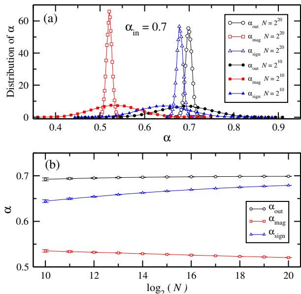
FIG. 2: (Color online) Finite size effects . (a) Distributions of \alpha_{out} , \alpha_{mag} and \alpha_{sign} for two ensembles of 65,000 series generated by using the Fourier Filtering Method with \alpha_{in} = 0.7 . Open symbols: length of the series N = 2^{20} \simeq 10^6 , full symbols: length of the series N = 2^{10} \simeq 10^3 . Due to statistical fluctuations, the values of the correlation exponent \alpha_{out} are not exactly equal to \alpha_{in} , instead they are normally distributed with a variance that decreases as N increases. A similar behavior is observed for \alpha_{mag} and \alpha_{sign} . (b) Mean values and standard deviations (error bars) of the distributions of \alpha_{out} , \alpha_{mag} and \alpha_{sign} for experiments similar to those in (a) for series size ranging from N = 2^{10} to N = 2^{20} . In all three cases the mean values seem to approach an asymptotic value as N grows. In particular, both \alpha_{out} and \alpha_{sign} tend to the same value, \alpha_{in} , the convergence being slower for \alpha_{sign} . The fact that \alpha_{out} and \alpha_{sign} have the same asymptotic limit is observed only within the region 0.5 \leq \alpha_{in} < 1 , whereas in the region \alpha_{in} > 1 , \alpha_{mag} tends asymptotically to the same limit as \alpha_{out} (see section III).
