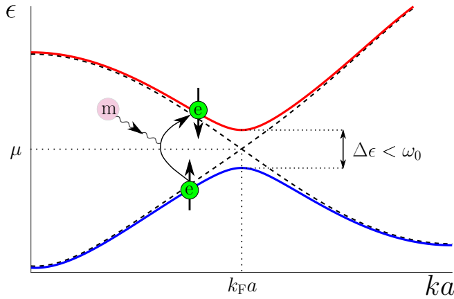
FIG. 3. A schematic depiction of magnon-induced interband scattering in a band (anti-)crossing at the Fermi level.
