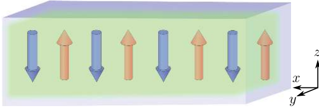
FIG. 1. Schematic depiction of our model for a metallic AFM. The red and blue arrows represent the localized d electrons with spin up and down, and constitute the Néel ordered magnetic subsystems. The green cloud illustrates the delocalized, itinerant s electrons that forms the conduction subsystem.
