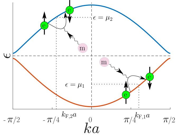
FIG. 2. The s electron dispersion in the metallic AFM model with illustrations of intraband electron-magnon scattering at two different Fermi levels, \mu_1 and \mu_2 . The depicted momentum transfer is exaggerated for clarity.
