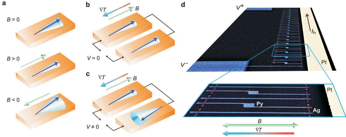
FIG. 1. Magnon-drag detection principle and geometry of the device. a , The magnon population in ferromagnetic wires is represented schematically by an arrow with a given precession angle. A magnetic field, B > 0 , applied parallel to the magnetization, leads to a reduction/damping of the magnon population (represented by a reduction in the precession angle). In contrast, a magnetic field B < 0 , antiparallel to the magnetization, results in an increase of the magnon population (increase in the precession angle). b , c , Magnon-drag measurements. The wires are connected thermally in parallel and electrically in series. For parallel magnetization orientation ( b ), the thermoelectric voltage is zero because the contribution from each wire is the same and has opposite sign. For the antiparallel configuration ( c ), in the presence of B , a nonzero thermoelectric voltage is measured due to the difference in magnon-drag effect, directly related to the difference in magnon populations induced by B . d , Scanning electron microscope image (SEM) of a typical device. A large number of pairs of NiFe wires (blue) are connected in series with Ag wires (red). A wide Pt wire (yellow) serves as a heater to generate a thermal gradient, \nabla T .
