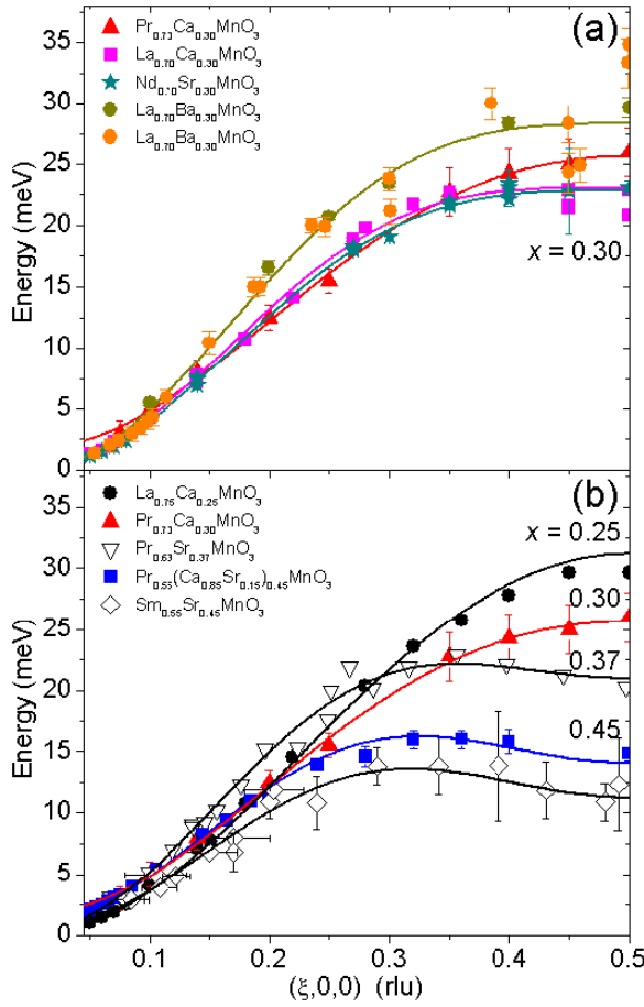
Figure 11. Summary of magnon dispersion curves along the [1, 0, 0] direction for (a) various R_{0.7}A_{0.3}MnO_3 manganites and (b) a series of R_{1-x}A_xMnO_3 as a function of x . The solids are the least-square fits using the Heisenberg model with J_1 and J_4 . Data are obtained from [19, 21, 24, 25, 27, 28, 32].
