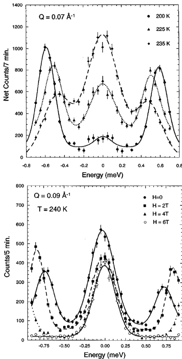
Figure 19. Top, T dependence below T_C = 250 K; bottom, field dependence at T = 240 K of magnetic inelastic neutron scattering spectra for the \text{La}_{2/3}\text{Ca}_{1/3}\text{MnO}_3 polycrystal. The figure is taken from [52]. The central peak is due to quasi-elastic spin diffuse scattering while the two side peaks are due to the magnon excitations. Similar results have been obtained from the \text{La}_{0.7}\text{Ca}_{0.3}\text{MnO}_3 single crystal [55]. The curves are fits to the data.
