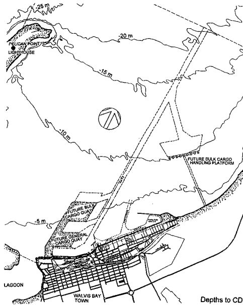
Figure 3: Proposed future extensions to the Port of Walvis Bay
