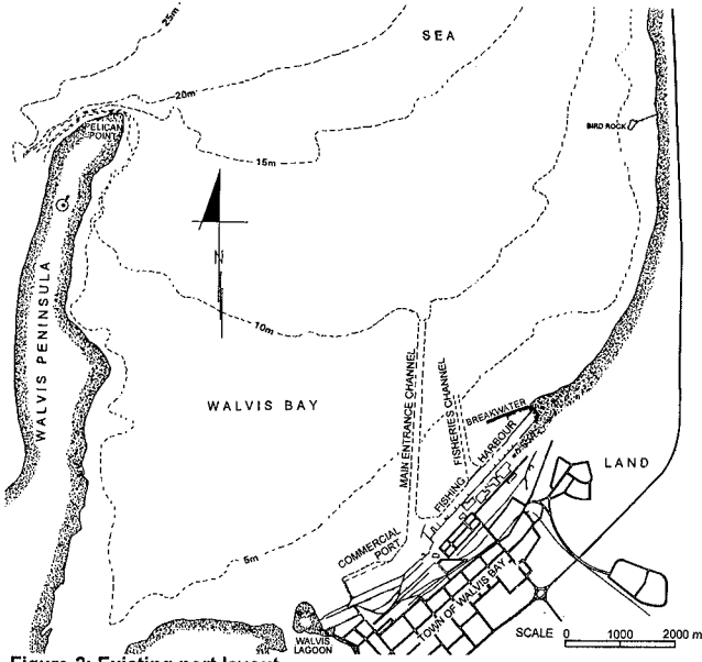
Figure 2: Existing port layout
