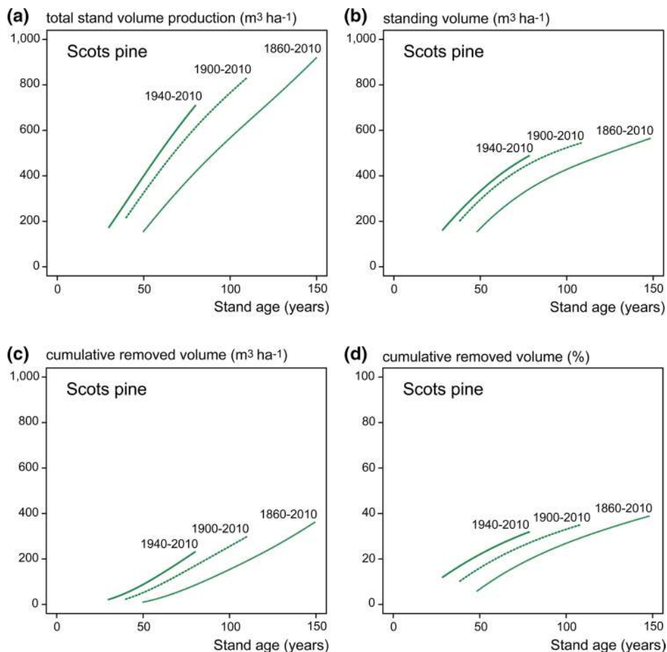
Fig. 15 Change in a total stand volume production, b standing volume, c accumulated removed volume and d percentage of removed volume of fully stocked, unthinned or just moderately thinned long-term experiments of Scots pine established in 1860, 1900, and 1940. Cumulated removed volume is the total production minus standing volume; the percentage of removed volume results from (total production - standing volume)/total production \times 100
