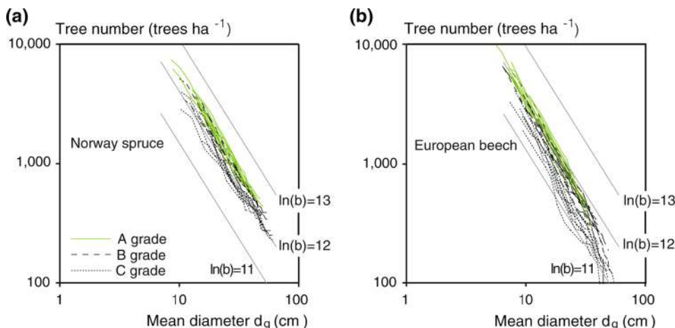
Fig. 4 Long-term development of tree number over mean tree diameter ( \ln(N) - \ln(d_q) -relationship) for thinning trials in even-aged stands of a Norway spruce (n=9) and b European beech (n=9) for untreated, fully stocked plots (A grade), medium (B grade) and strong thinning (C grade). Reference lines \ln(N) = \ln(b) - 1.605 \times \ln(d_q) in accordance with Reineke (1933) where \ln(b) = 11, 12, 13 (after Pretzsch and Biber 2005)
