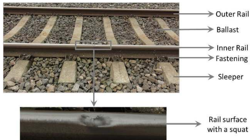
Figure 1.1: A severe squat on the rail surface.
