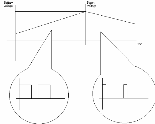
Fig 3 Current waveform of VPWC
