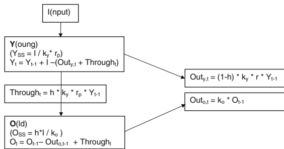
Fig. 1 Structure of the Introductory Carbon Balance Model (ICBM) by Andren and Kätterer (1997). State variables are Y_t and O_t , representing a young, unstable and an old, stable organic N pool respectively ( \text{kg ha}^{-1} ) and their steady state condition ( Y_{SS} and O_{SS} , respectively, \text{kg ha}^{-1} ), k_y and k_o are decomposition rates for the young and old pool respectively ( \text{kg ha}^{-1} \text{ year}^{-1} ), h is the humification factor (-), r_p is the “ploughing” coefficient (-). Through_t is an internal flux, the throughput of N from the young to the old pool ( \text{kg ha}^{-1} \text{ year}^{-1} ). External fluxes are Out_{y,t} , Out_{o,t} , the N release by the young and old N pools respectively ( \text{kg ha}^{-1} \text{ year}^{-1} ). t represents time (year)
