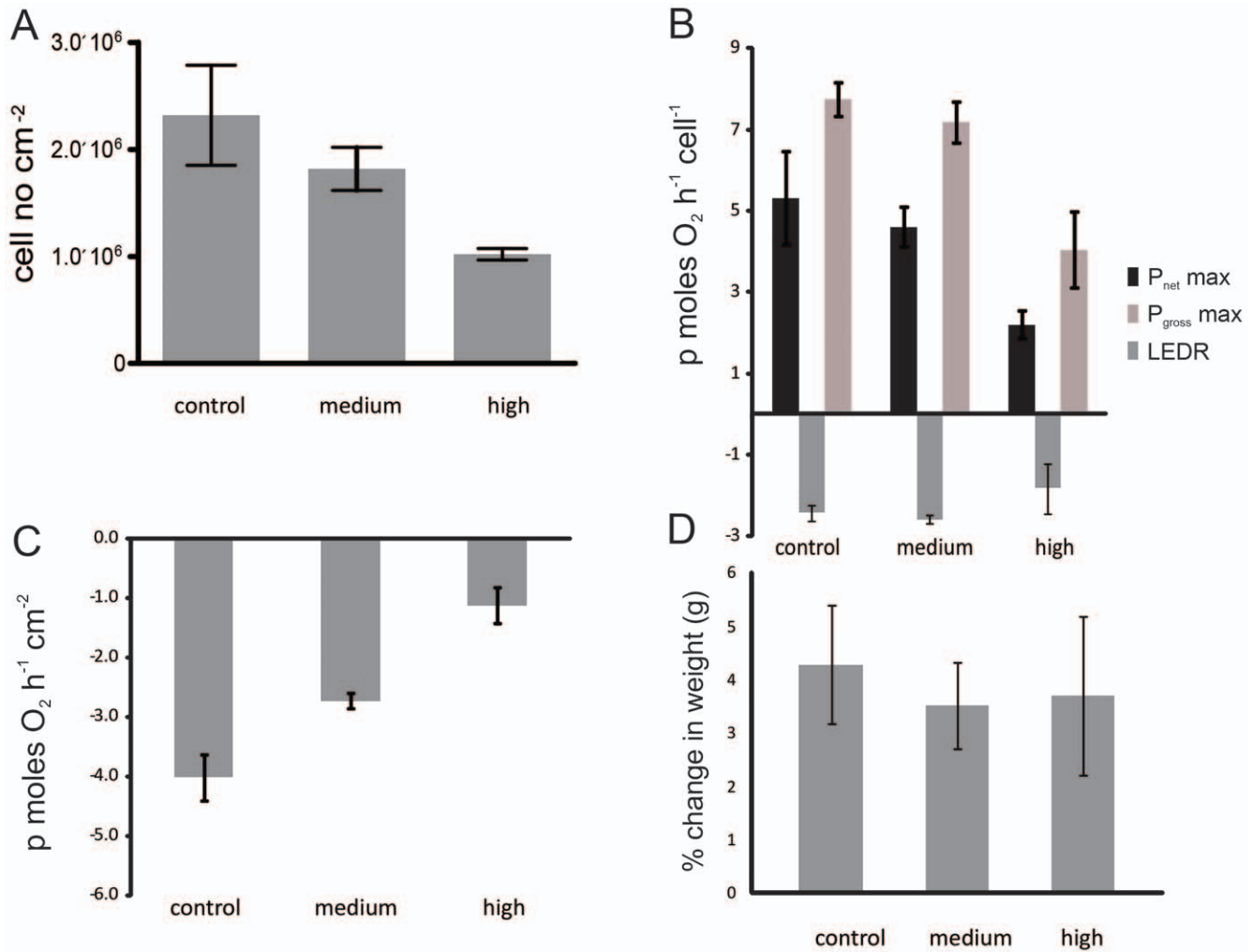
Figure 4. The effect of increasing CO 2 in seawater (control, medium and high) after 28 days on coral-algal physiology. (A) Symbiodinium cell number in reef-building coral, Acropora millepora (B) photosynthetic capacity per symbiont cell measured as P net max, light enhanced dark respiration (LEDR), and P gross max (P net max - LEDR) (C) dark respiration (R dark ) and (D) relative calcification/growth as % change in weight (g) of coral branches over the 28 day experimental period. Error bars represent the standard error of the mean (n=4). doi:10.1371/journal.pone.0034659.g004
