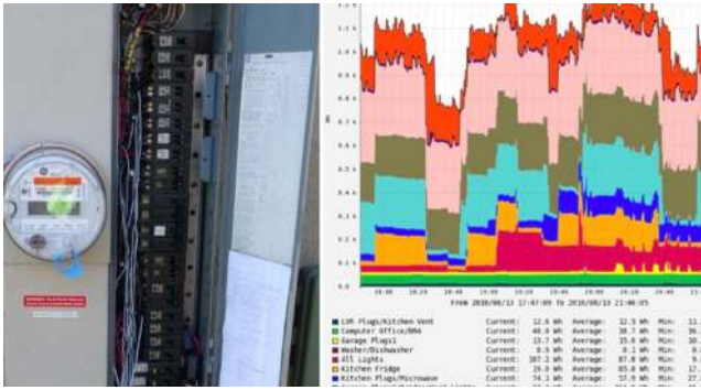
Figure 3. Irwin's home-brewed electricity use monitoring system.
