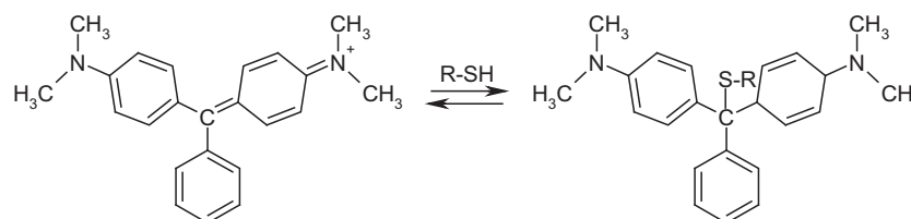
Figure 7: Proposed scheme of malachite green adduct formation with thiols
