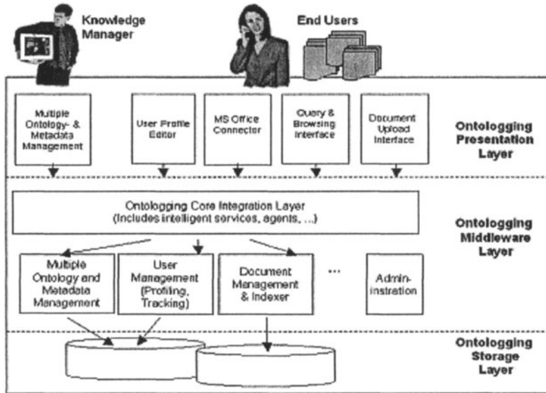
Figure 1. Overall Ontologging Architecture
