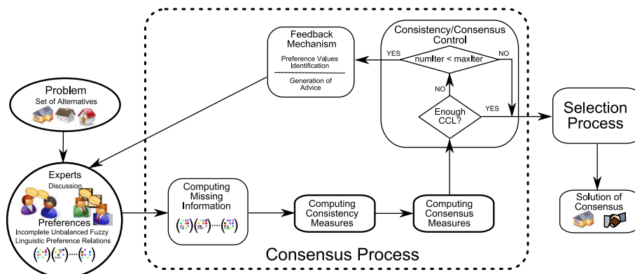
Fig. 4. Scheme of consensus model.
