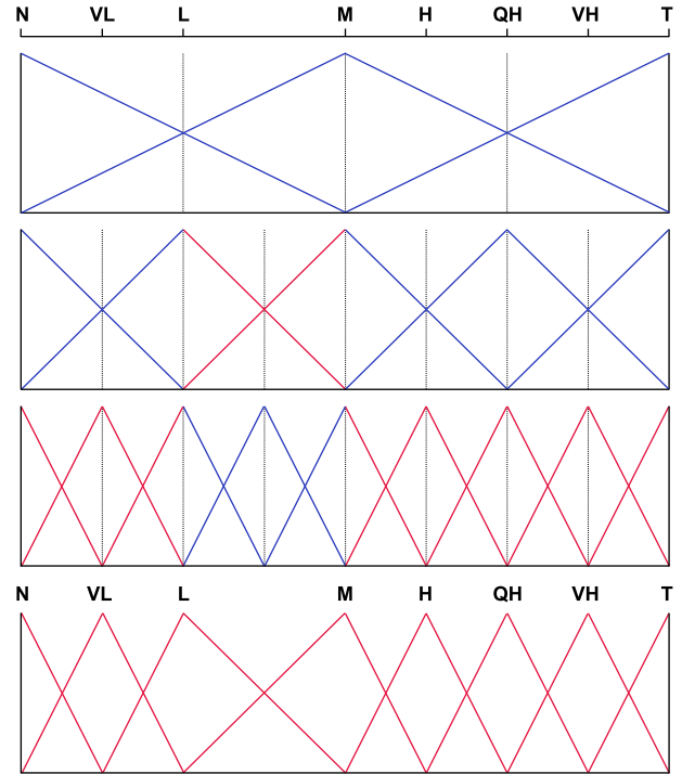
Fig. 3. Representation for an unbalanced linguistic term set of 8 labels using a linguistic hierarchy.
