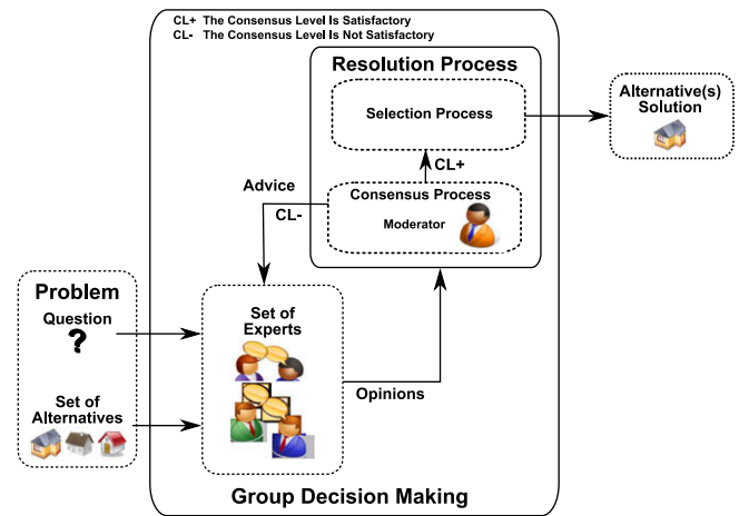
Fig. 2. Resolution process of a GDM problem.
