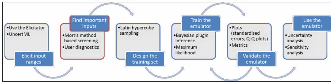
Figure 6. The main steps in constructing an emulator. For each stage, including the optional screening step, the methods supported within UncertWeb are listed.
