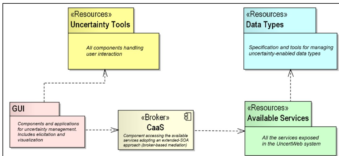
Figure 2 Dependency view of the main UncertWeb architectural components.
