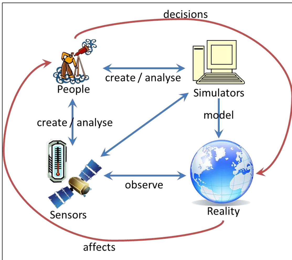
Figure 1. A schematic representation of the relation between people, reality, models and observations.
