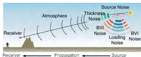
Fig. 1. Rotorcraft acoustics issues.
