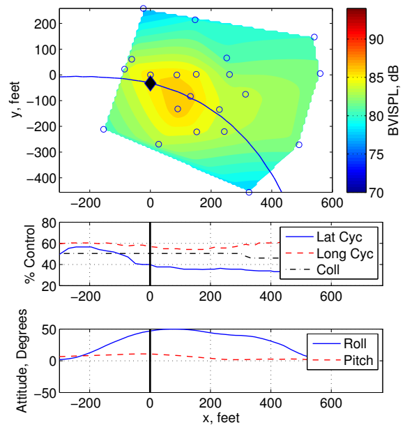
Fig. 28. Right roll during 9° climb.
