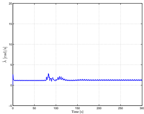
Fig. 6. The dynamic variable \dot{\lambda} remains uniformly ultimately bounded.
