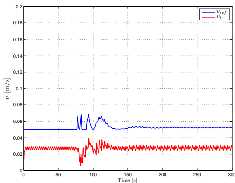
Fig. 8. Reference and actual tangential velocities.
