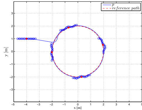
Fig. 3. Plots of the snake robot with 10 links and the path of its center of mass. An animation can be found at https://www.youtube.com/watch?v=Bkqi9AcbSo .
