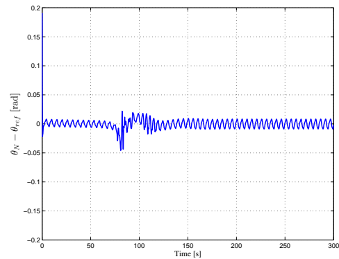
Fig. 9. The head angle tracking error.
