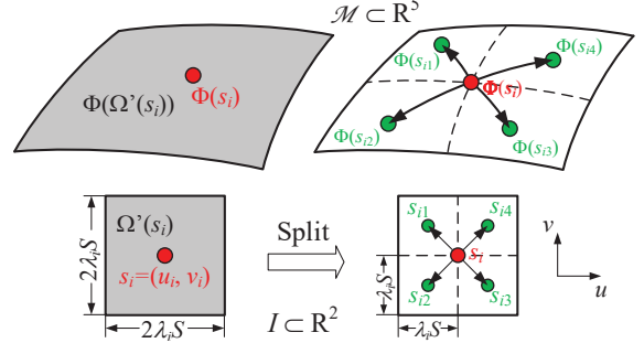
Figure 4. Illustration of the splitting operator. \Omega'(s_i) is a 2\lambda_i S \times 2\lambda_i S region on the image I around s_i . If Area(\Phi(\Omega'(s_i))) > 4\Xi (i.e., \lambda_i < 0.5 ), where \Xi = 4Area(\mathcal{M})/K is a fixed area of a local search region in image manifold \mathcal{M} , the splitting operator replaces s_i = (u_i, v_i) into four new generators s_{i1} = (u_i - \frac{\lambda_i S}{2}, v_i + \frac{\lambda_i S}{2}) , s_{i2} = (u_i - \frac{\lambda_i S}{2}, v_i - \frac{\lambda_i S}{2}) , s_{i3} = (u_i + \frac{\lambda_i S}{2}, v_i - \frac{\lambda_i S}{2}) and s_{i4} = (u_i + \frac{\lambda_i S}{2}, v_i + \frac{\lambda_i S}{2}) . We set the adaptive scaling factors as \lambda_{i1} = \lambda_{i2} = \lambda_{i3} = \lambda_{i4} = \lambda_i/2 .
