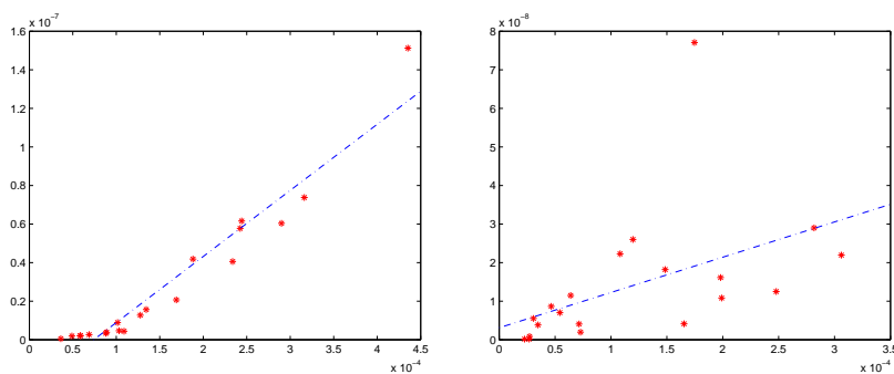
Fig. 4. Vertebrae outlines: Projection difference \tau_{S_{\hat{v}}} as a function of the indicator \tilde{\tau}_{S_{\hat{v}}} (left) and residual difference \rho as a function of the indicator \sigma (right).
