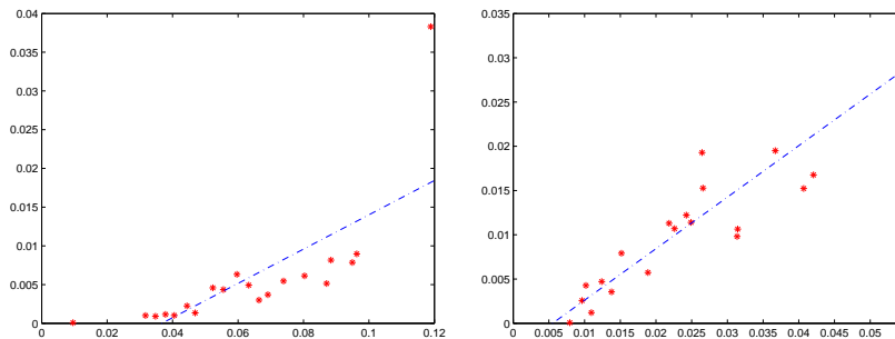
Fig. 6. Human poses: Projection difference \tau_{S_{\hat{\sigma}}} as a function of the indicator \tilde{\tau}_{S_{\hat{\sigma}}} (left) and residual difference \rho as a function of the indicator \sigma (right).
