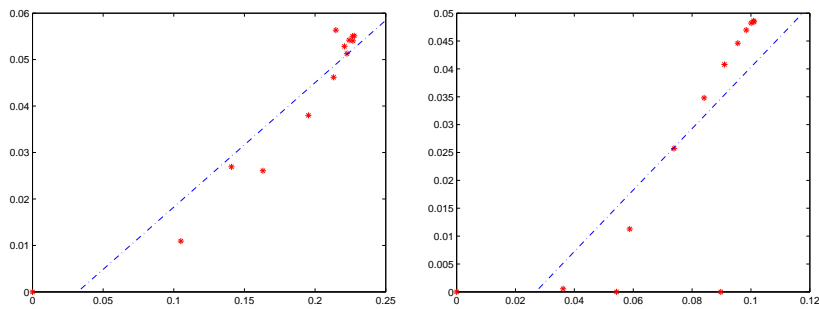
Fig. 2. Synthetic data: Projection difference \tau_{S_{\hat{v}}} as a function of the indicator \tilde{\tau}_{S_{\hat{v}}} with the broken line fitted to the points (left) and residual difference \rho as a function of the indicator \sigma with the broken line fitted to the points (right).
