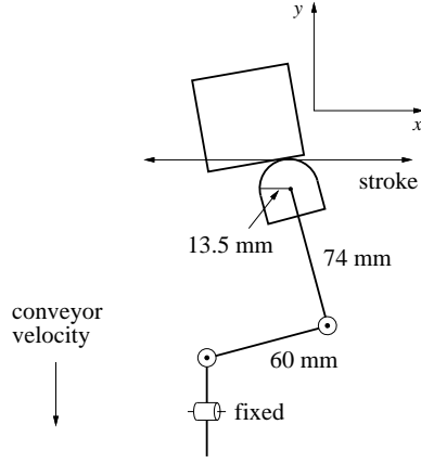
Fig. 5. Experimental setup.
