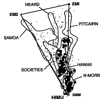
Fig. 3. "Side" view (as in Fig. 1B), showing the Hawaiian and N-MORB fields (and several others for comparison). The Hawaiian array does not appear to be mixing toward N-MORB, but instead is apparently aiming to the left of the general N-MORB field. The N-MORB field scatters around the DMM-EM1-HIMU base triangle, suggesting possible contamination of DMM with EM1 and HIMU, but not with EM2.
