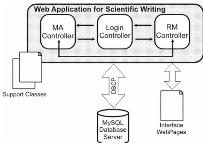
Figure 2 Manuscript Architect architecture.
