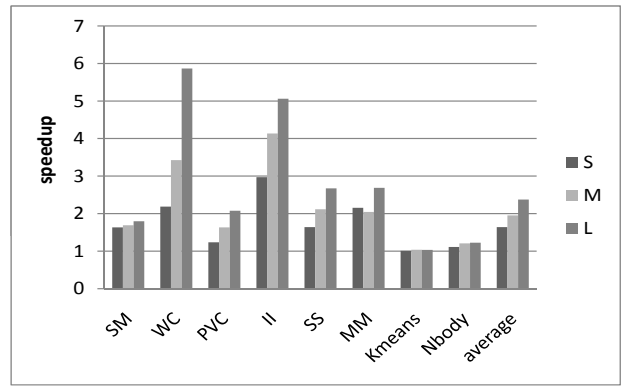
Figure 9: Speedup of MapCG over Mars on GTX280 GPU, using Small, Medium, and Large datasets.
