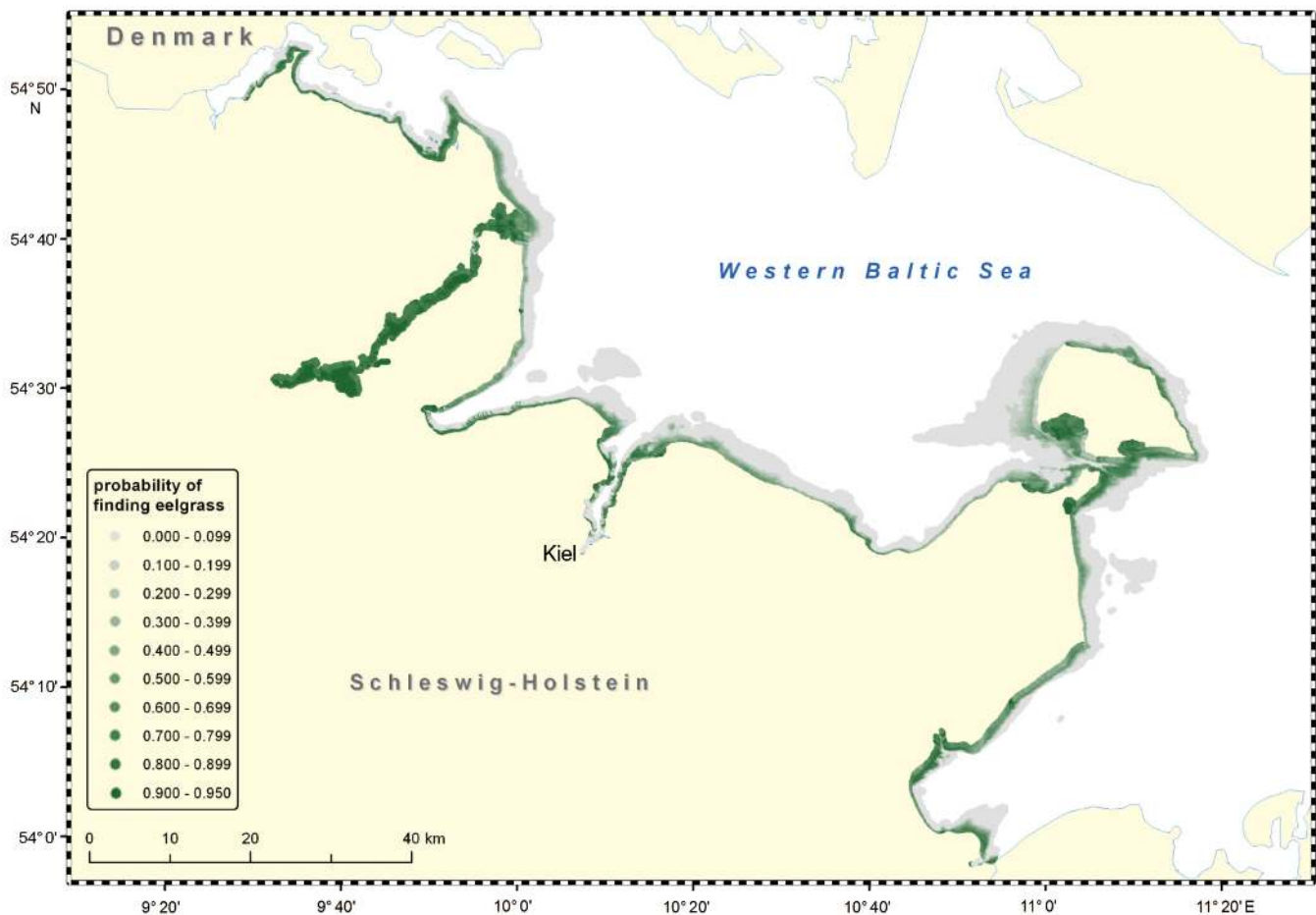
Fig. 5. Predicted probability of eelgrass occurrence along the coast of Schleswig-Holstein for the final model (Model 1). The darker green the area, the larger the probability to find eelgrass. Horizontal resolution of the model is 100 m; maximum depth is 10 m
