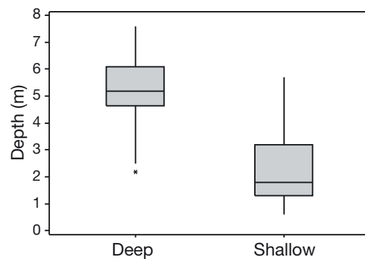
Fig. 3. Box plot of depth limit range for deep and shallow depth limits along perpendicular mapping transects with eelgrass ( n = 97 ), showing median (centre line), 1st to 3rd quartiles (box limits), range of values (whiskers) and outliers (*)
