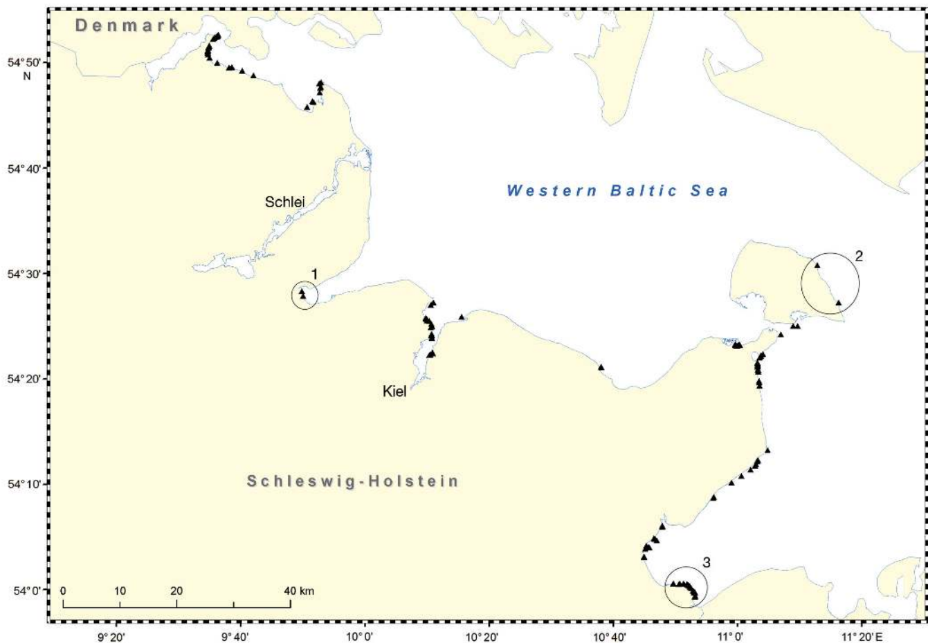
Fig. 6. Falsely predicted presences (with 5% probability of error in predicting the presence of eelgrass) for the final model (Model 1). Small triangles show locations where eelgrass is absent, although the modeled probabilities to find eelgrass are high (>0.77). Circles ring potential restoration sites (1: Eckernförde Bay; 2: Fehmarn-East; 3: Brodten Cliff). The Schlei Fjord was excluded from the analysis
