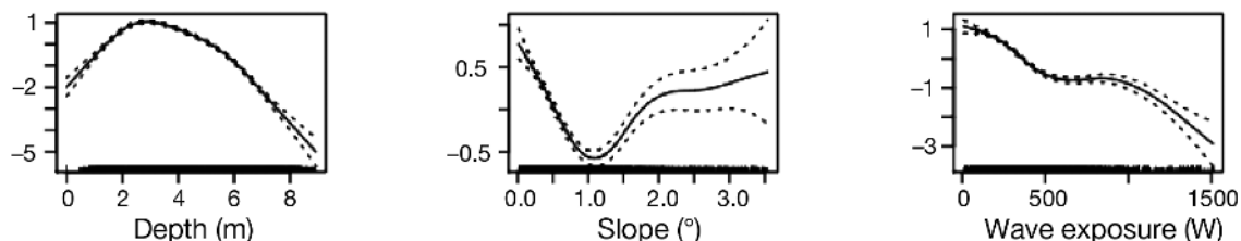
Fig. 4. Response curves of eelgrass presence/absence to the predictor variables depth, slope, and wave exposure in the generalized additive model analysis for the final model (Model 1). The y-axis represents the additive contribution of each variable (range differs between panels). Black ticks above x-axis represent observation range. Dashed lines represent 95% confidence interval limits
