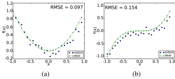
Fig. 7: Computing mathematical functions with neurons. (a) computed function f(x) = x^2 , RMSE = 0.097 . (b) computed function f(x) = x^3 , RMSE = 0.154 .
