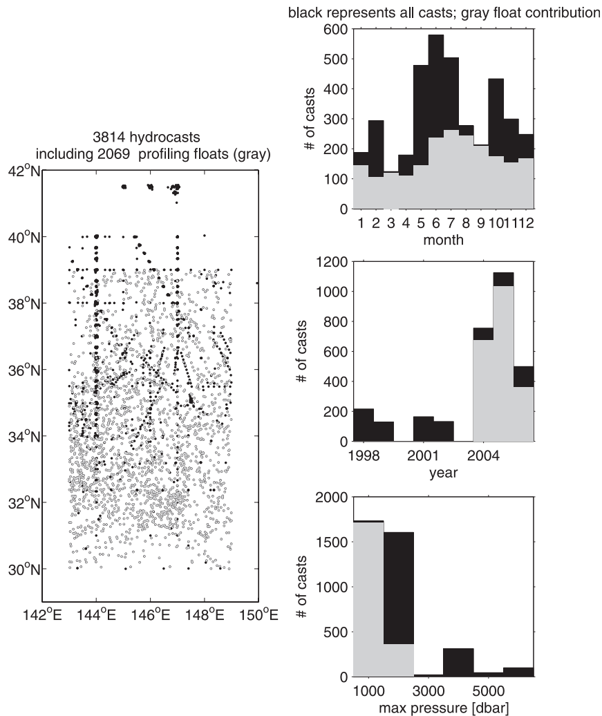
FIG. 9. Hydrographic dataset used to construct the seasonal cycle, the GEM lookup table, and the conversion between \tau_{\text{index}} and measured \tau . (right) Histograms of (top) cast month, (middle) year, and (bottom) pressure. Float profiles—represented by (left) gray dots and (right) gray bars—constitute a large fraction of the dataset. (left) Map of station locations.
