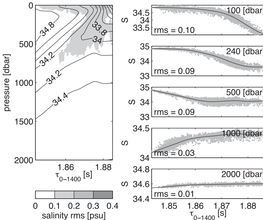
FIG. 12. As in Fig. 11, but for salinity.
