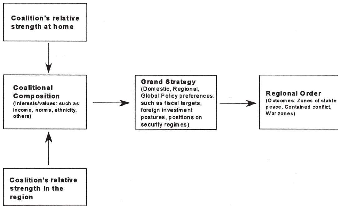
FIG. 2. Causal logic.
