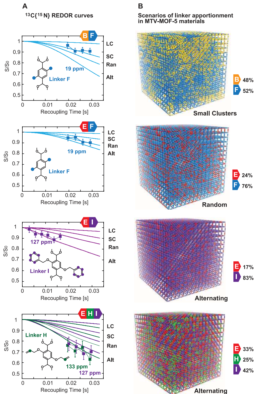
Fig. 3. REDOR results and apportionments. (A) Experimental ^{13}\text{C}\{^{15}\text{N}\} REDOR curves (squares) are compared with the molecular dynamics simulations for the different linker apportionments, large clusters (LC), small clusters (SC), random (Ran), and alternating (Alt). (B) The derived apportionments for the different MTV-MOF-5s. Yellow, linker B; blue, linker F; red, linker E; purple, linker I; green, linker H.
