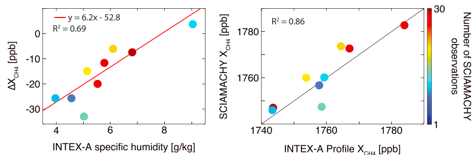
Figure 2. Validation of the SCIAMACHY IMAP v5.5 retrieval of methane column mixing ratio ( X_{CH_4} ) with coincident INTEX-A aircraft vertical profiles (see text). (left) Difference \Delta X_{CH_4} between SCIAMACHY and INTEX-A plotted as a function of the mean pressure-weighted specific humidity in the 900–400 hPa column measured by the INTEX-A aircraft. The red line shows a linear regression weighted by the number of SCIAMACHY observations. Regression parameters and weighted R^2 are shown inset. (right) Comparison of SCIAMACHY and INTEX-A X_{CH_4} after applying the water vapor correction from the linear regression. Weighted R^2 is shown inset, and the 1:1 line is also shown. Colors represent the number of SCIAMACHY observations averaged around each INTEX-A profile.
