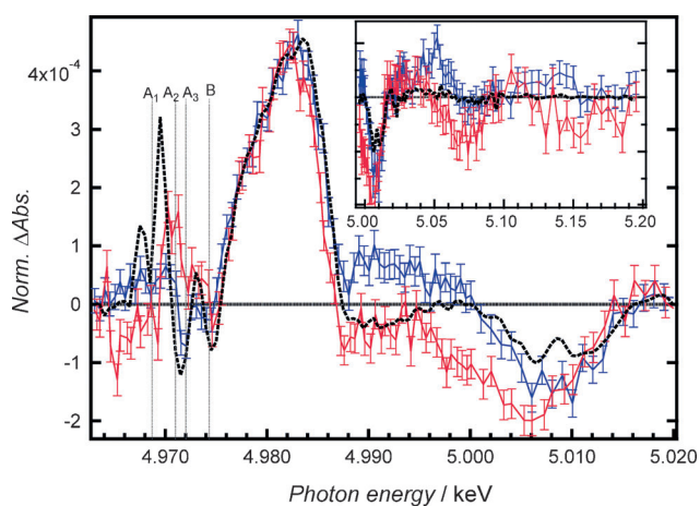
Figure 2. Normalized transient spectra at a time delay of 100 ps of bare amorphous NPs excited at 355 nm (blue) and N719-dye-sensitized amorphous NPs, excited at 532 nm (red). The black dashed line represents the static difference spectrum obtained by subtracting the measured steady-state spectrum from the steady-state spectrum shifted by -1 eV and normalization to the transients at 4.981 keV. The inset shows the above-edge region of the same transient spectra.
