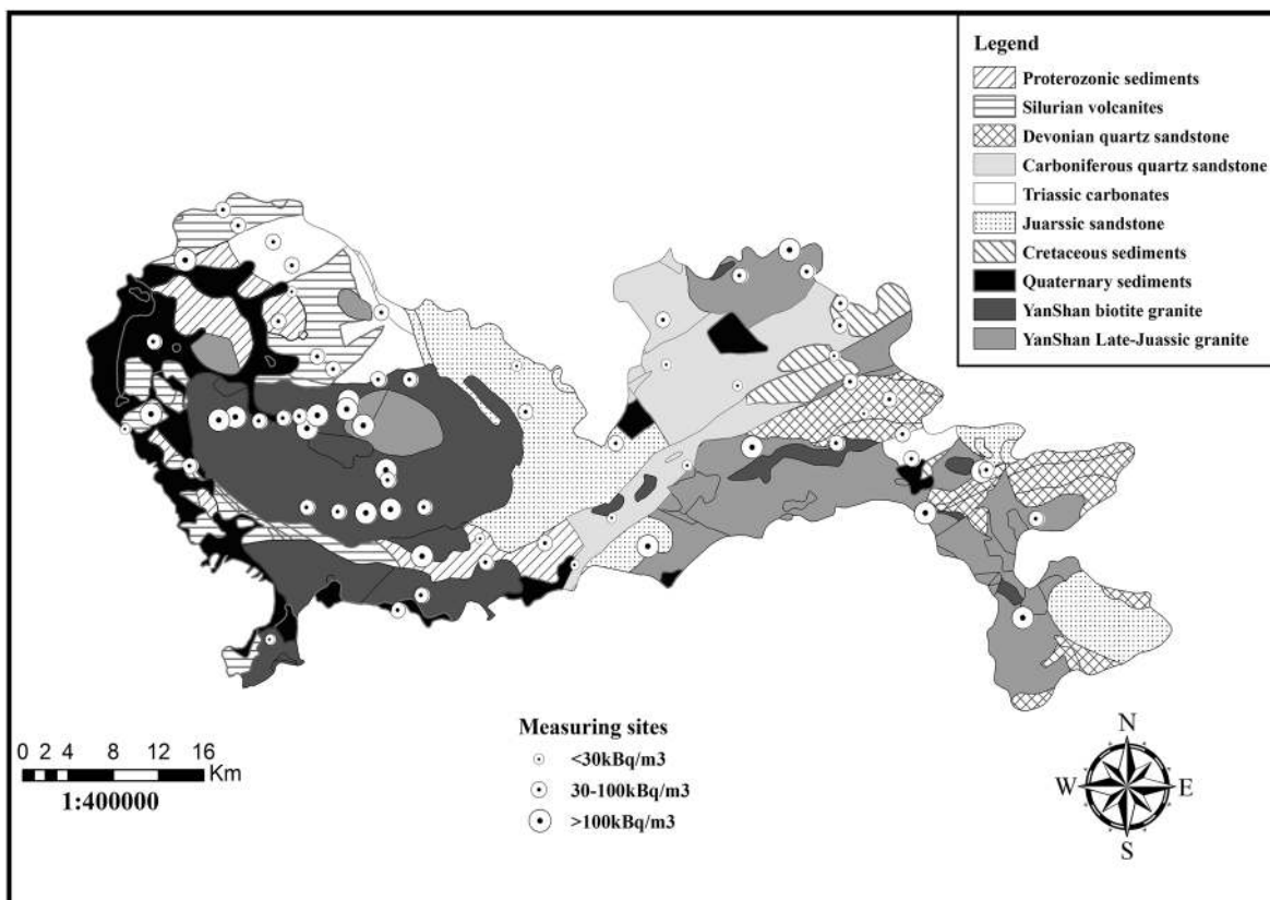
Fig. 2 The geological sketch map of Shenzhen City with the distribution of measuring sites [size of dot represents the different range of soil gas radon concentration (kBq/m 3 )]
