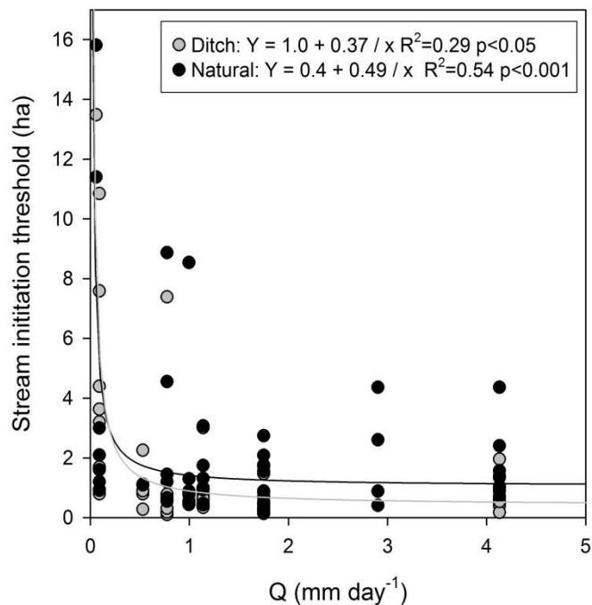
Figure 2. Stream initiation threshold area (ha), also known as channelization threshold or source area, for the stream heads of natural streams and ditches, respectively. The dots denote field measurements on till soils during different flow situations (Q), i.e. , how much land area (ha) is needed before a stream develops.
