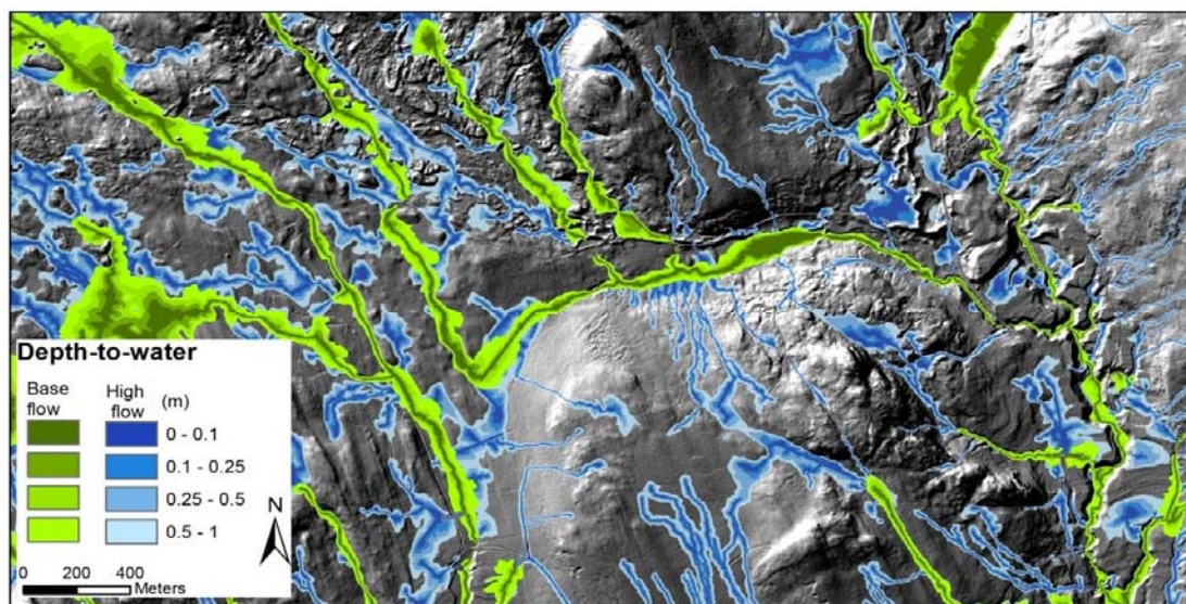
Figure 5. The black and white background map shows the sunlit elevation model of a subsection of the Krycklan catchment. Superimposed are the depth-to-water index maps which mark the wet areas along the stream network. Blue areas indicate wet areas during spring flood and green areas indicate areas that remain wet during baseflow. The darker colors (blue or green) indicate that the modelled groundwater level is closer to the soil surface and hence wetter.
