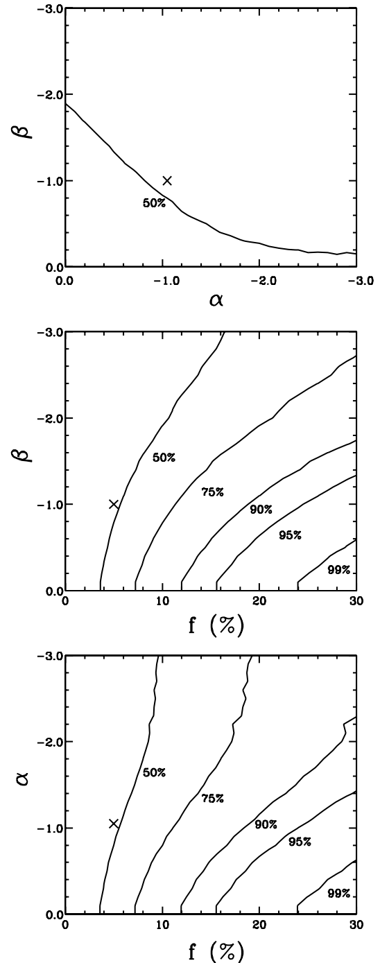
FIG. 7.—Our survey's joint limits on the total giant planet frequency f , the mass function power law \alpha , and the semimajor axis distribution power law \beta , assuming that we fix each parameter at the canonical value suggested by RV surveys (e.g., Marcy et al. 2005): f = 5\% (top), \alpha = -1.05 (middle), and \beta = -1.0 (bottom). In each case, we also denote the confidence level corresponding to all three canonical values with crosses. [See the electronic edition of the Journal for a color version of this figure.]
