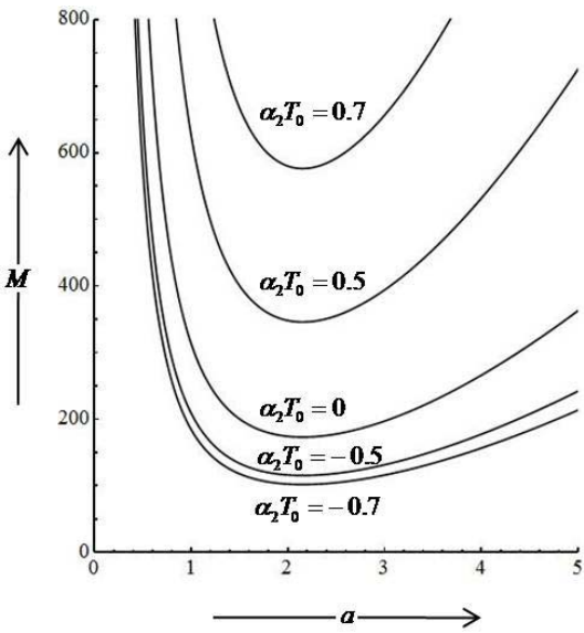
Fig.1c. Neutral stability cuwes for various values of \alpha_2 T_0 when L=4 .
