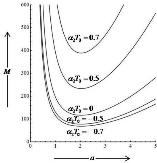
Fig.1b. Neutral stability cuwes for various values of \alpha_2 T_0 when L=2 .
