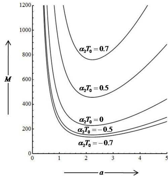
Fig.1d. Neutral stability cuwes for various values of \alpha_2 T_0 when L=6 .
