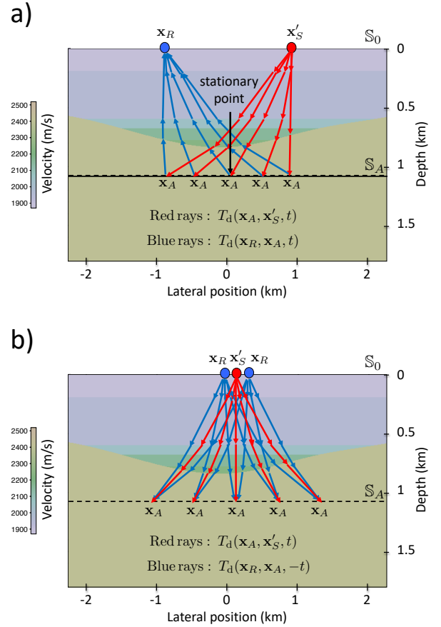
FIG. 10 (a) Visualization of equation 53. Convolution of the transmission responses yields a reflection response (the ray via the stationary point). (b) Visualization of equation 54. Correlation of the transmission responses yields a band-limited focus around \mathbf{x}'_S .
