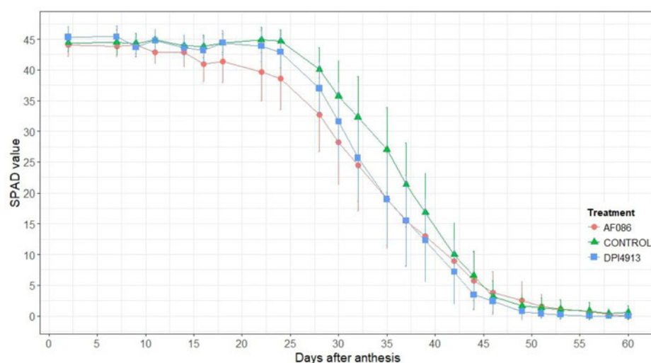
Fig. 1. Changes in SPAD values in flag leaves after anthesis under different treatments (greenhouse experiment). Biostimulants were applied at the second node stage.
