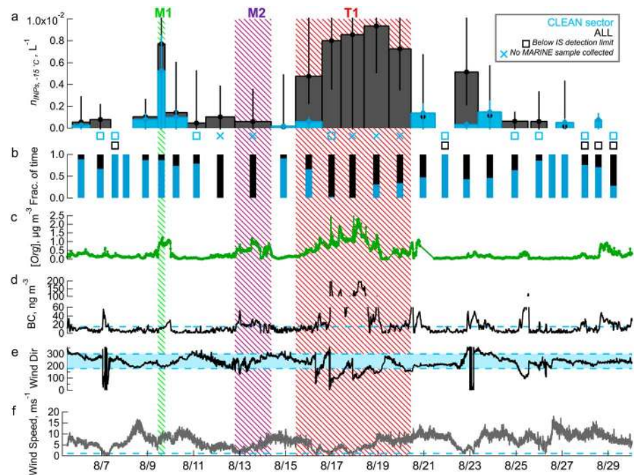
Figure 1. (a) Timeline of INP number concentrations active at -15^{\circ}\text{C} ( n_{\text{INPs},-15^{\circ}\text{C}} ) for ALL (black) and CLEAN sector (blue) samples. Open square markers indicate measured n_{\text{INPs},-15^{\circ}\text{C}} that were below detection limit. Cross markers indicate that a sample was not collected for that sampling period. Vertical bars are the 95% confidence intervals for IS measurements. (b) Fraction of sampling time that was in the CLEAN sector (blue) versus nonclean sectors (black). Timeline of (c) organic carbon mass concentrations measured by the HR-ToF-AMS, (d) equivalent black carbon (eBC) mass concentrations, (e) wind direction (Wind Dir), and (f) wind speed. Green, purple, and red shadings correspond to organic events M1, M2, and T1. In d and e, thresholds used to define CLEAN sector periods are shown in light blue for eBC, wind direction, and wind speed. INP = ice-nucleating particle; BC = black carbon.
