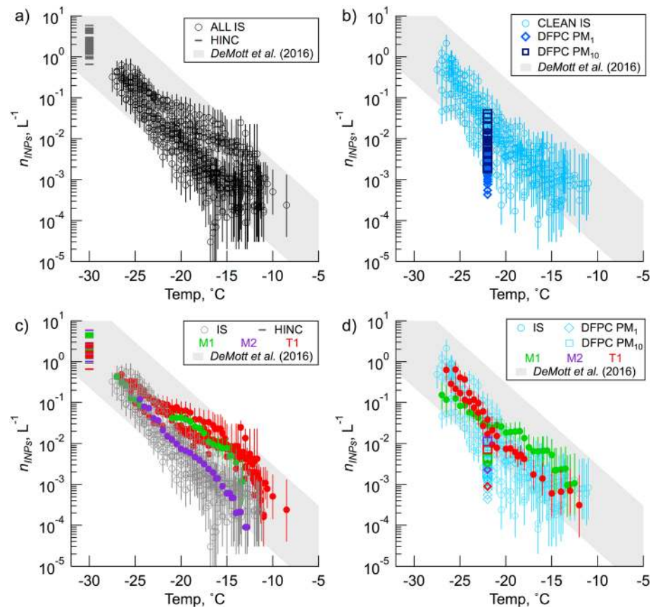
Figure 4. INP temperature spectra for (a) ALL samples, (b) CLEAN sector samples, (c) ALL samples with highlighted events, and (d) CLEAN sector samples with highlighted events. Data include those from IS (circles), HINC-EV (dash markers), DFPC PM 1 (diamond markers), and PM 10 (squares). In (c), grey open circles correspond to ALL aerosol for a given collection period. In (d), light blue open circles correspond to aerosol collected in the CLEAN sector only. In (c) and (d), green, purple, and red filled circles correspond to the INP concentrations measured by the IS during the M1, M2, and T1 organic events, respectively. HINC-EV and DFPC are also highlighted for each organic event. The light grey shaded area represents the range of values reported by DeMott et al. (2016) for nascent laboratory-generated and ambient SSA. INP = ice-nucleating particle; IS = Ice Spectrometer; HINC-EV = Horizontal Ice Nucleation Chamber-Evaporation; DFPC = Dynamic Filter Processing Chamber; SSA = sea spray aerosol.
