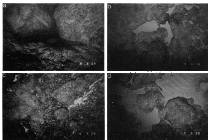
Fig. 4. (a to d) Bottom photographs (width \sim 2 m) of sea-floor crusts and pavements on Horizon Seamount ( 19^{\circ}30'N , 169^{\circ}W ; depth \sim 1290 m) [photographs by H. Chezar (23)]. (e) Continuous ferromanganese cobbles and pavement on the Blake Plateau, off the Southeast Atlantic margin of the
