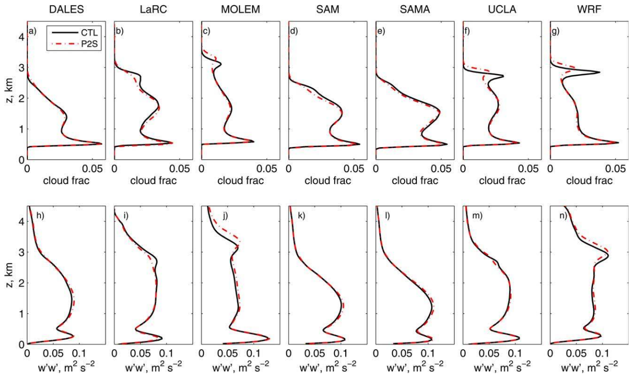
Figure 22. Time-averaged profiles of (a-g) cloud fraction and (h-n) vertical velocity variance for the S6 control and P2S sensitivity studies from the CGILS LES intercomparison are shown from (a,h) DALES, (b,i) LaRC, (c,j) MOLEM, (d,k) SAM, (e,l) SAMA, (f,m) UCLA, and (g,n) WRF.
