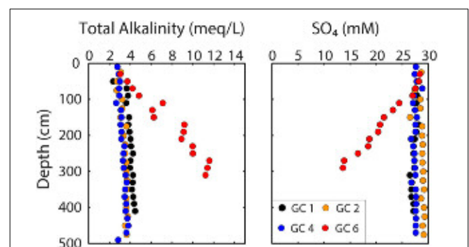
FIGURE 8 | Pore water profiles of total alkalinity [from Devey et al. (2018)] and \text{SO}_4 along an E-W transect on the Vema TFFZ (for locations see Figure 9 ).
