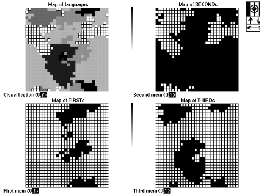
Fig. 3: Distribution of languages and features after 150 steps.
