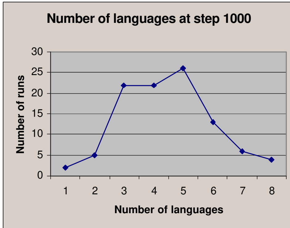
Figure 6: Distribution of languages after 1000 steps
