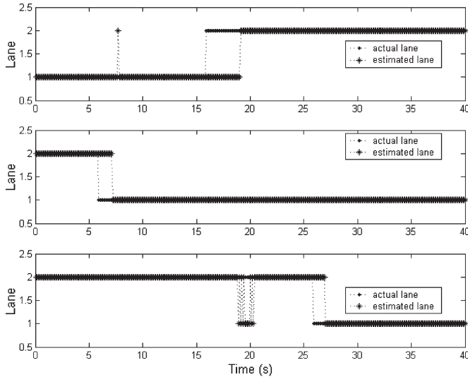
Fig. 9. Impact of oscillatory weaving (car 1 to car 3 from top to bottom): This figure shows a simulation in which car 1, car 2, and car 3 follow sinusoidal paths with different amplitudes (−1, −1, and 1 m) and frequencies (1/4, 1/4.5, and 1/5 Hz).
