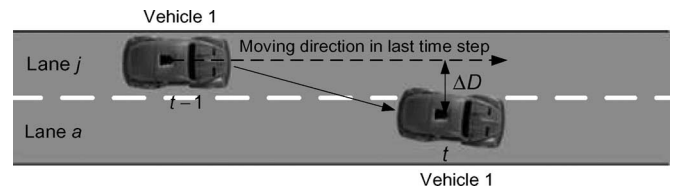
Fig. 2. Prediction step: This figure illustrates a vehicle (with an unknown position) switching lanes. The shortest distance \Delta D from the position estimate at time t to the line passing through the two most recent position estimates is used to calculate the conditional probability.
