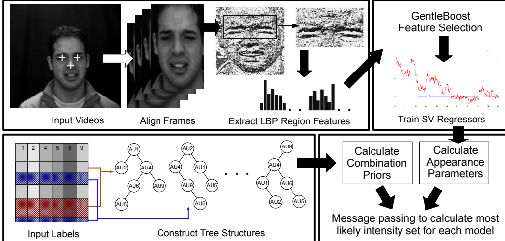
Figure 3. An overview of our full system.
