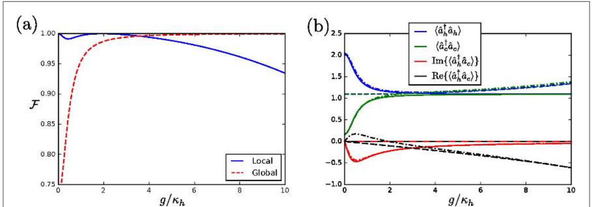
Figure 5. Comparison of steady states out of equilibrium obtained from the local master equation (see equation (12)), the global master equation (see equation (23)), and exact numerics. (a) Fidelity between the states obtained from the master equation and the state obtained from exact numerics. The dip in the fidelity for the local approach occurs at g \approx |\Sigma_h| and is therefore assumed to arise from neglecting the renormalization of the Hamiltonian; see equation (16). (b) Other observables as a function of interaction strength. Solid: local master equation, dashed: global master equation, dashed-dotted: exact numerics. The global approach breaks down for small values of g . However, for large g , it gives a better prediction of the steady state than the local approach. Parameters: \Omega_h = 2 , \Omega_c = 1 , \kappa_h = \kappa_c = 0.05 , k_B T_c = 0.5 , k_B T_h = 5 . Parameters numerics: \omega_c = 3 , n = 400 , t = 20/\kappa .
