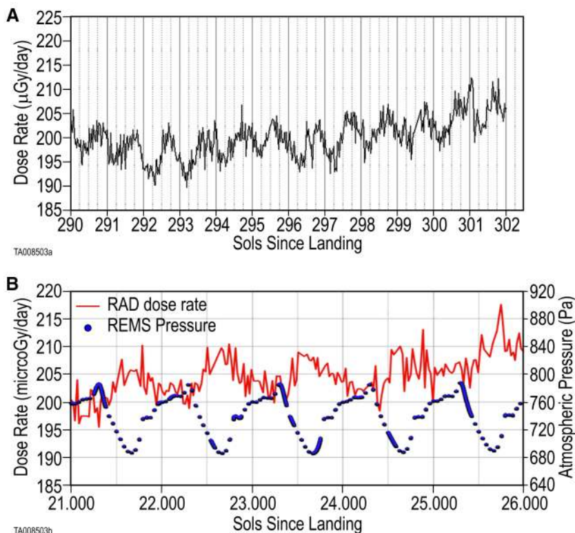
Fig. 2. Comparison of RAD dose rate versus time and atmospheric pressure. (A) RAD daily dose rate versus time. (B) Comparison of RAD dose rate with REMS atmospheric pressure.
