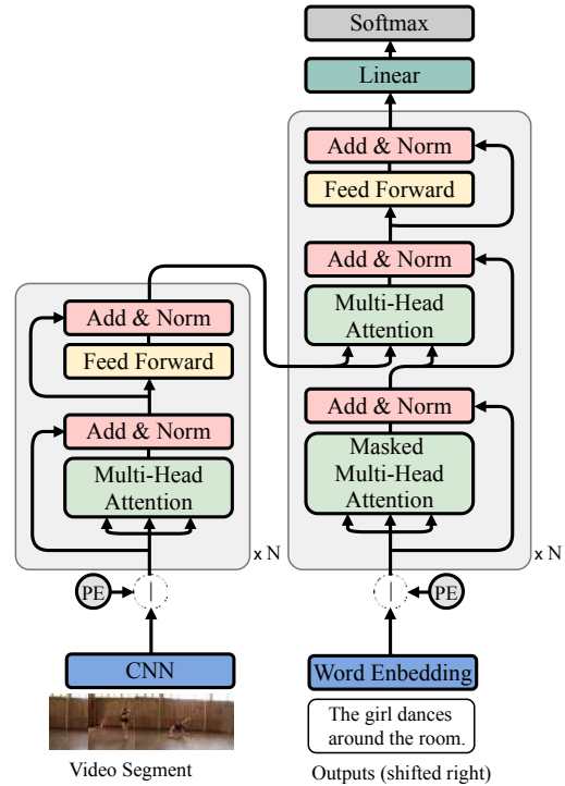
Figure 1: Vanilla transformer video captioning model (Zhou et al., 2018). PE denotes Positional Encoding, TE denotes token Type Embedding.
