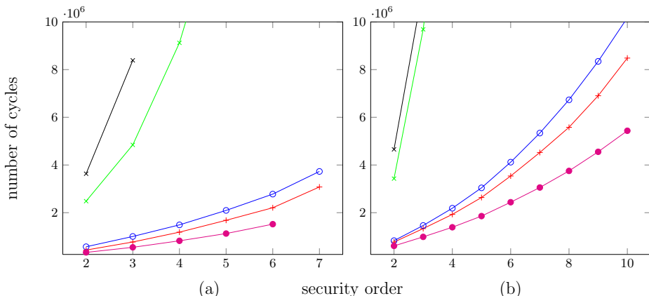
Fig. 1. Cycle counts for masked AES implementations: unrolled codes (a) and compact codes (b). The curves \text{---}\times\text{---} are for KHL , the curves \text{---}\times\text{---} are for RocP , the curves \text{---}\circ\text{---} are for RivP , the curves \text{---}\times\text{---} are for RocP* , and the curves \text{---}\bullet\text{---} are for GPQ .
