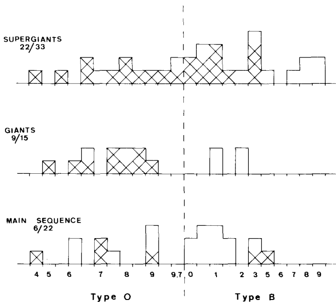
Fig. 1. Distribution of spectral types of program stars. For each luminosity class the ratio of the number of stars with substantial infrared excess (crosses) to the total, is given.
